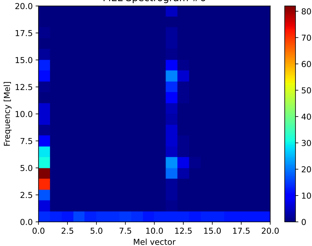
MEL Spectrogram #6
